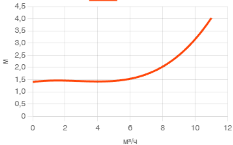
NPSH
