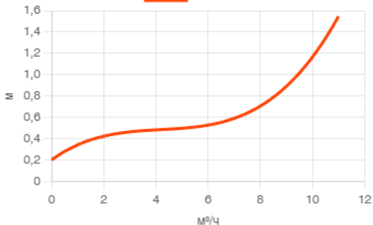
NPSH
